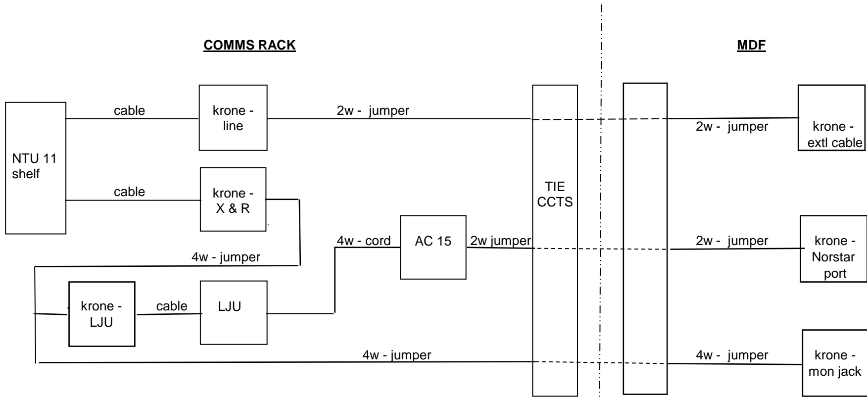
Connection of trunk circuits
